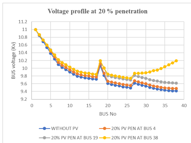
Figure 3: Voltage profile at 20% penetration
