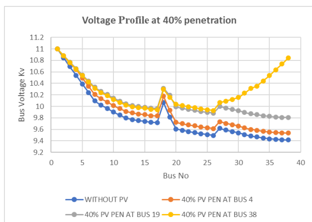
Figure 5: Voltage profile at 40% penetration
