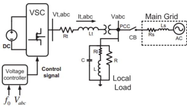
Figure 1: Isolated Operation of Inverter based DERs
