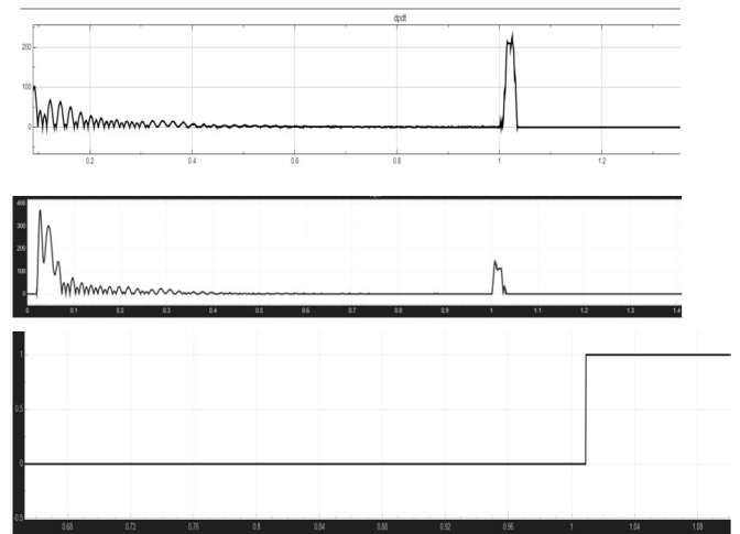
Figure 6: ROCOAP, ROCORP and trip Signal-Case-3
