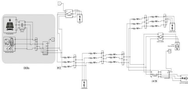
Figure 2: 11kV system and DERs connection test frame
