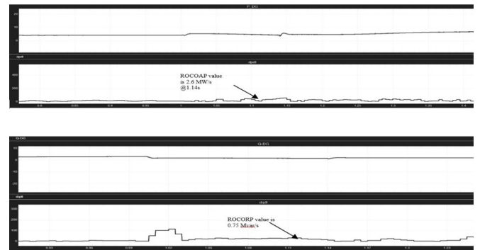
Figure 7: ROCOAP, ROCORP Plot
