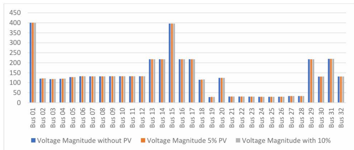
Figure 4: Voltage magnitude at different PV penetration levels.
