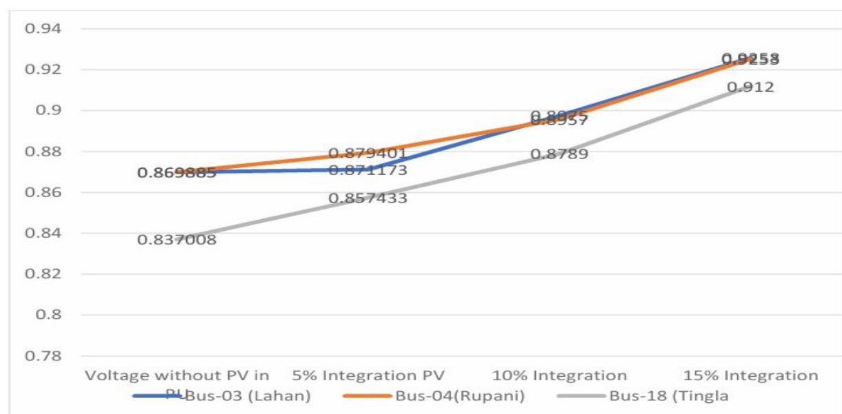
Figure 5: Voltage profile comparison of Bus-03 (Lahan), Bus-04 (Rupani), and Bus-18 (Tingla) under 5%, 10%, and 15% PV penetration levels.
