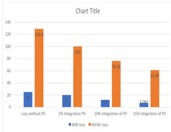
Figure 6: Comparison of power loss at different PV integration levels.
